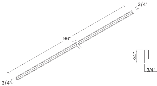
96" COVE CROWN MOLDING WITH CLEAT
