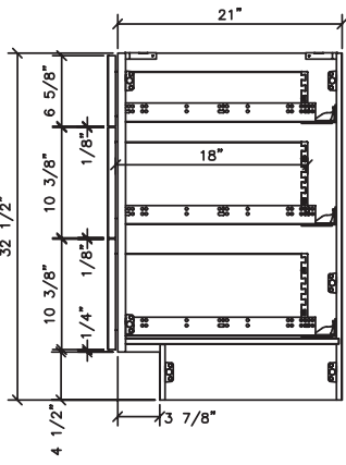
VDB15 ADA VANITY 3 DRAWER CABINET
