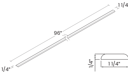
96" SCRIBE MOLDING
