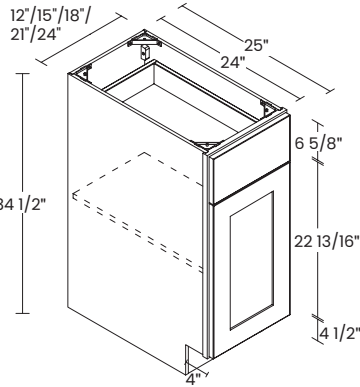
12", 15", 18", 21", 24" 1 DOOR / 1 DRAWER
