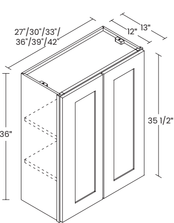
36" HIGH 2 DOORS
