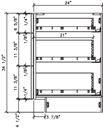
DB15 BASE 3 DRAWER CABINET
