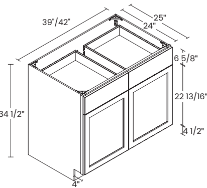
39", 42" 2 DOORS / 2 DRAWERS
