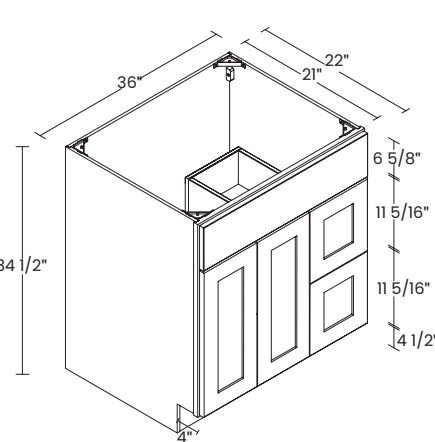
36" VANITY SINK BASE 2 DOORS / 2 DRAWERS / 1 FALSE FRONT
