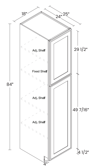
84" HIGH UTILITY CABINET WITH 2 DOORS, 1 FIXED SHELF AND 3 ADJUSTABLE SHELVES
