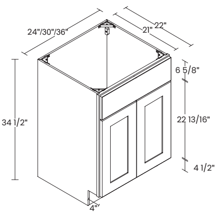
24", 30", 36" VANITY SINK BASE 2 DOORS / 1 FALSE FRONT
