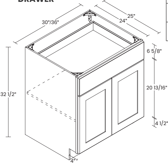
30", 36" BASE 2 DOORS / 1 DRAWER
