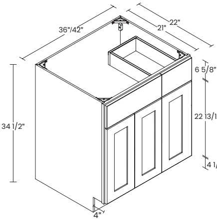
36", 42" VANITY SINK BASE 3 DOORS / 1 DRAWER / 1 FALSE FRONT
