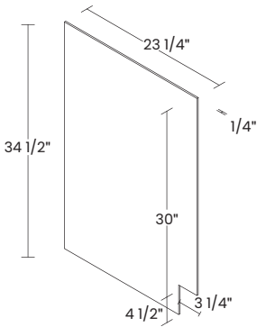
24" BASE END PANEL
