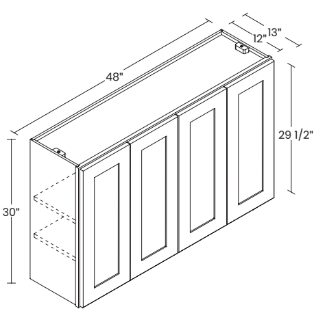
30" HIGH 4 DOORS
