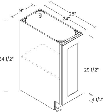
9" FULL HEIGHT 1 DOOR
