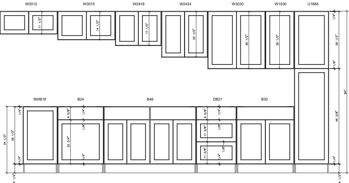
84" ASSEMBLED CABINETS
