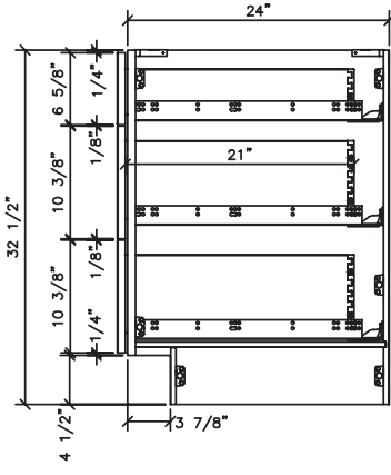
DB15 ADA BASE ADA 3 DRAWER CABINET
