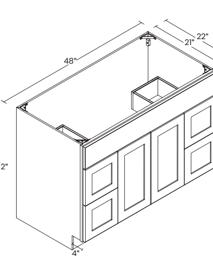
48" VANITY SINK BASE 2 DOORS / 4 DRAWERS / 1 FALSE FRONT
