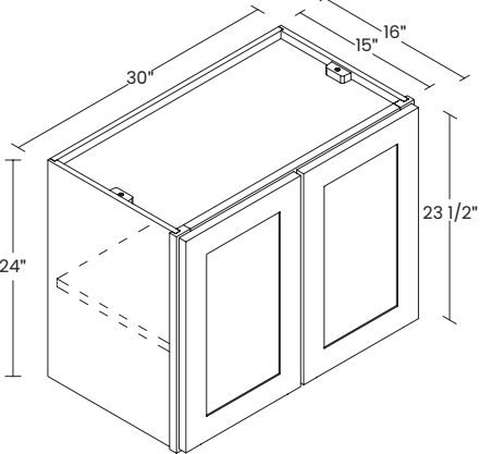
30" 2 DOORS
