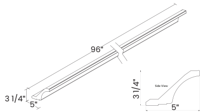
96" COVE CROWN MOLDING WITH CLEAT
