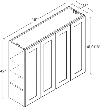
42" HIGH 4 DOORS
