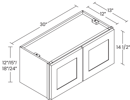
30" 2 DOORS
