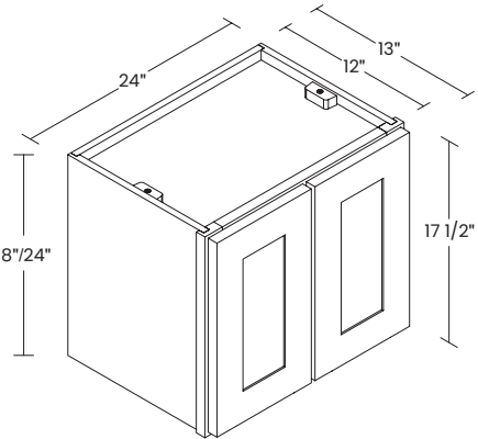
24" 2 DOORS
