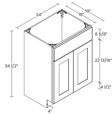
24" VANITY SINK BASE 2 DOORS / 1 FALSE FRONT
