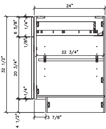
B15 BASE ADA CABINET
