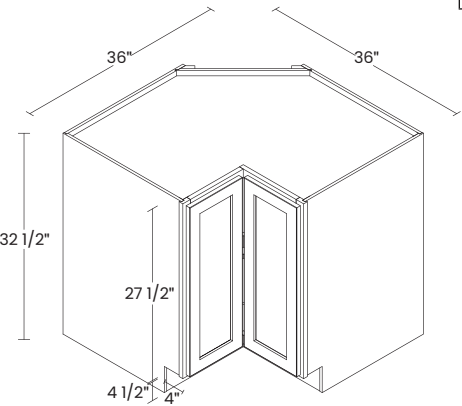
36" BASE CORNING CABINET WITH DURABLE POLYMER LAZY SUSAN
