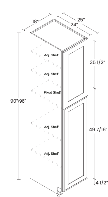
90", 96" HIGH UTILITY CABINET WITH 2 DOORS, 1 FIXED SHELF AND 4 ADJUSTABLE SHELVES
