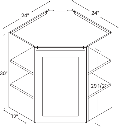
30" HIGH WALL DIAGONAL CORNER
