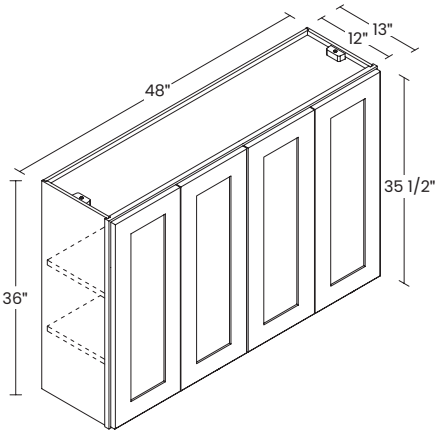
36" HIGH 4 DOORS
