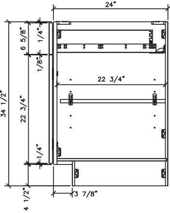
B15 BASE CABINET
